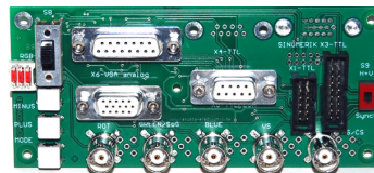
Connector panel
